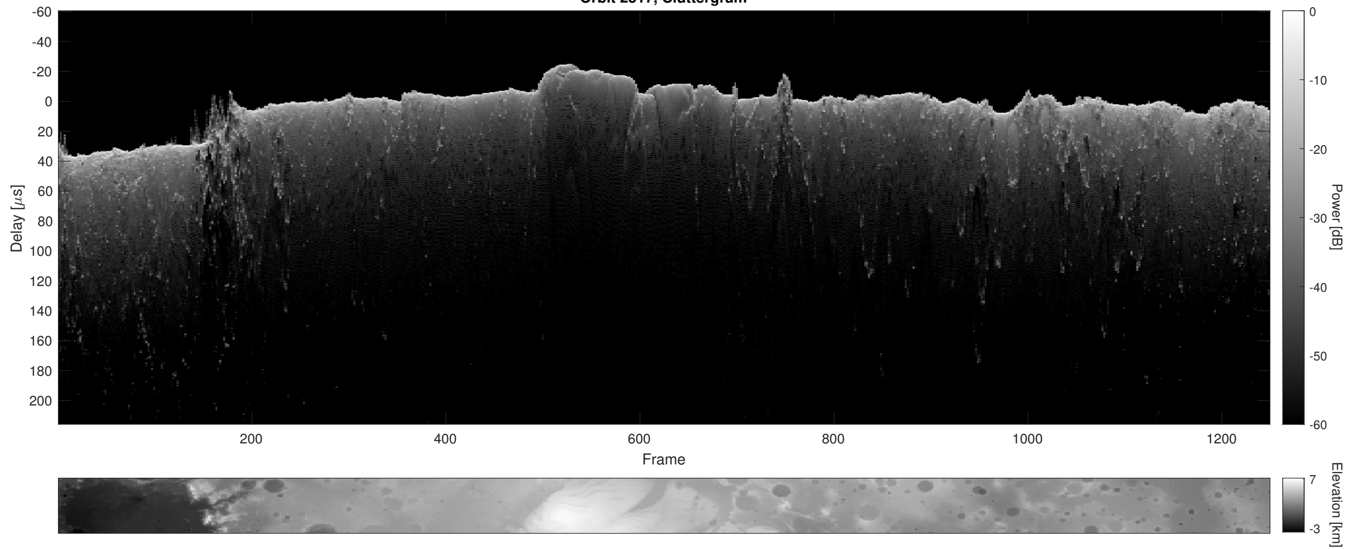
Orbit 2517, Cluttergram
