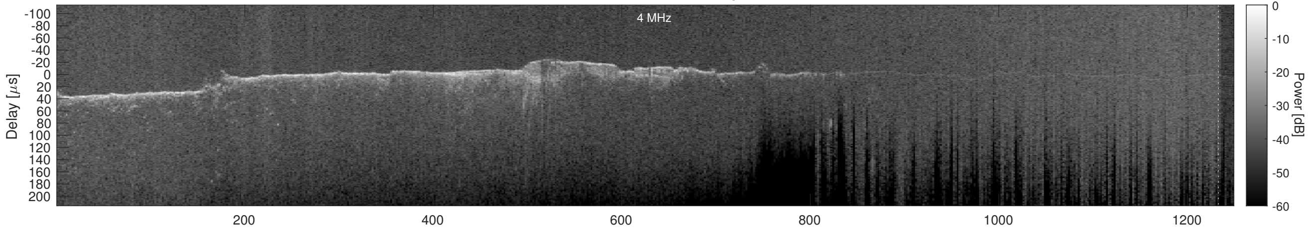
Orbit 2517, Cluttergram
