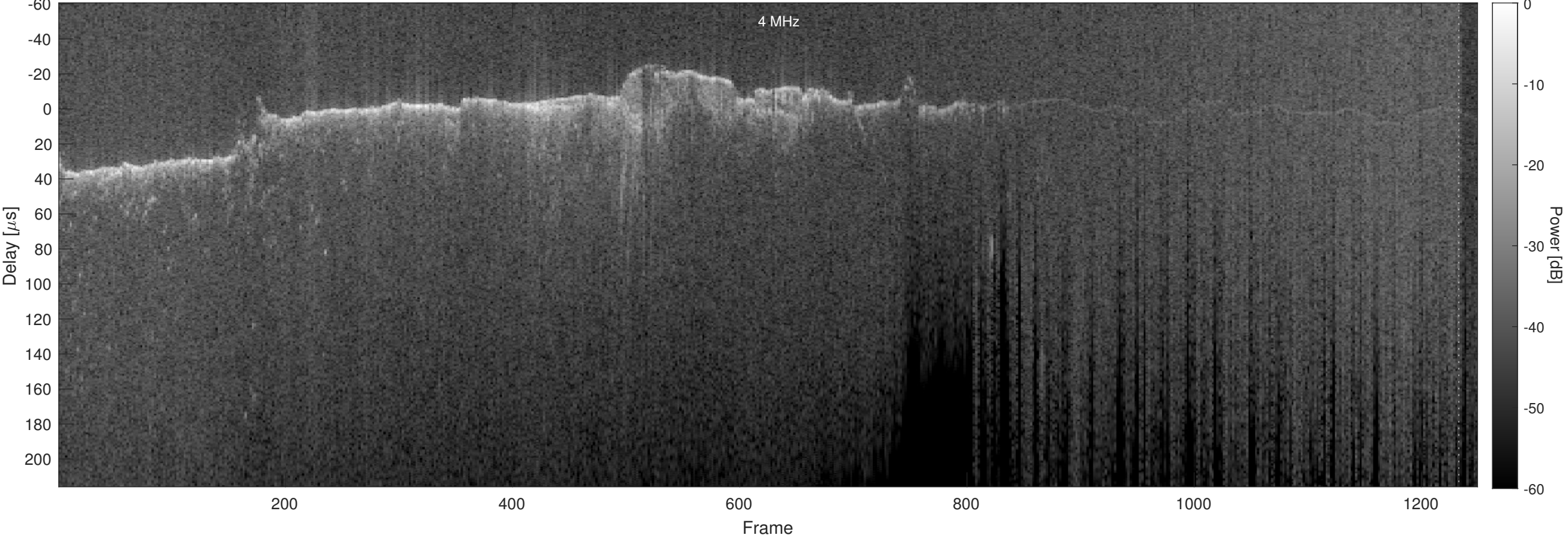
Orbit 2517, Optimized, No Window, Channel 2
