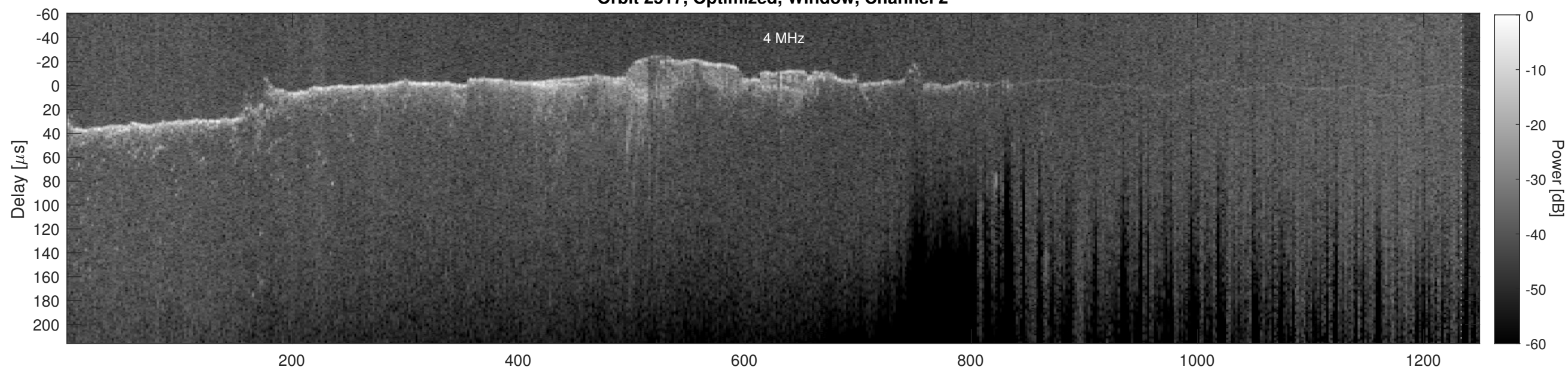
Orbit 2517, Cluttergram
