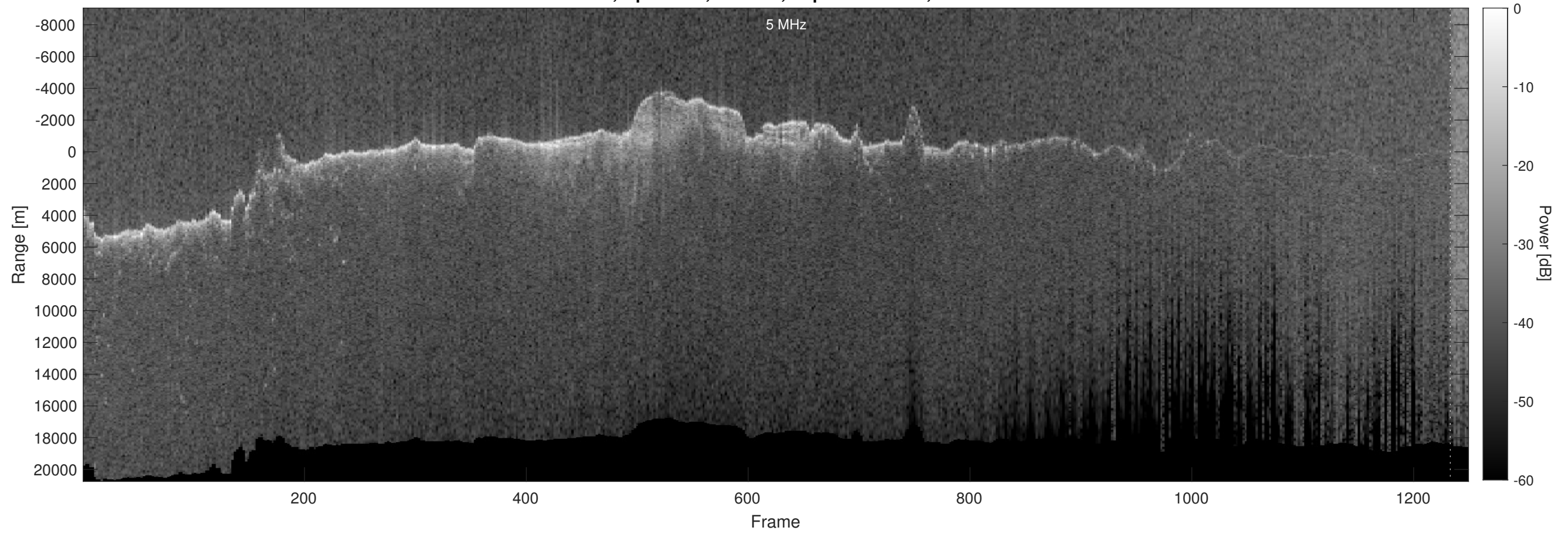
Orbit 2517, Optimized, Window, Depth-Corrected, Channel 2
