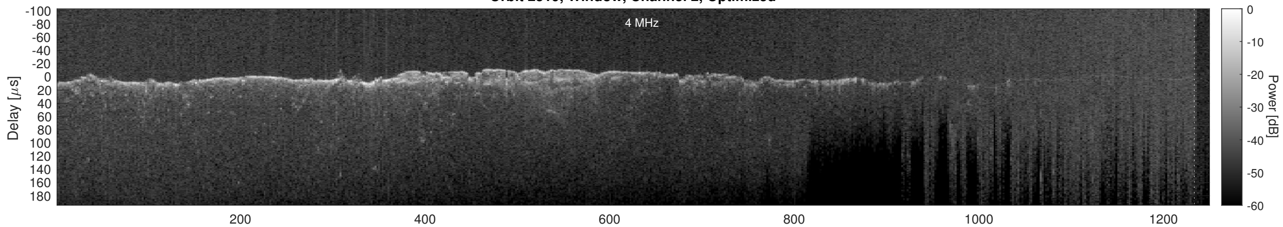
Orbit 2519, Cluttergram
