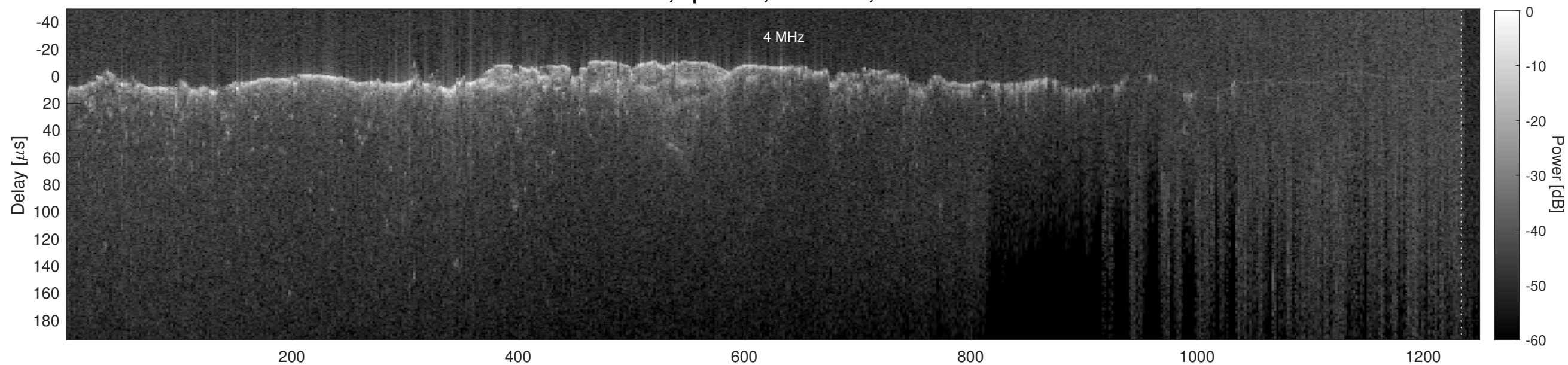
Orbit 2519, Cluttergram
