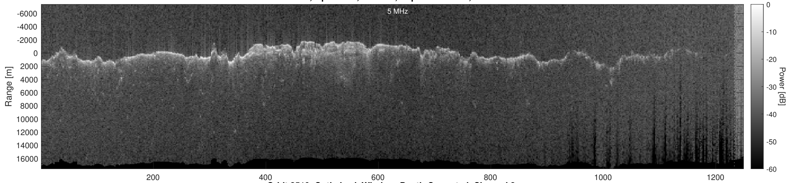
Orbit 2519, Optimized, Window, Depth-Corrected, Channel 2
