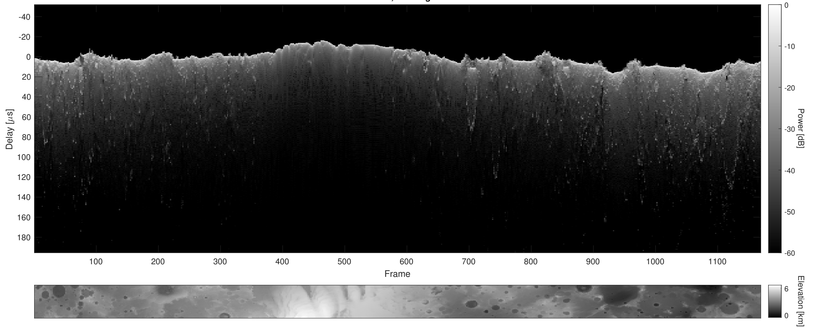
Orbit 2520, Cluttergram
