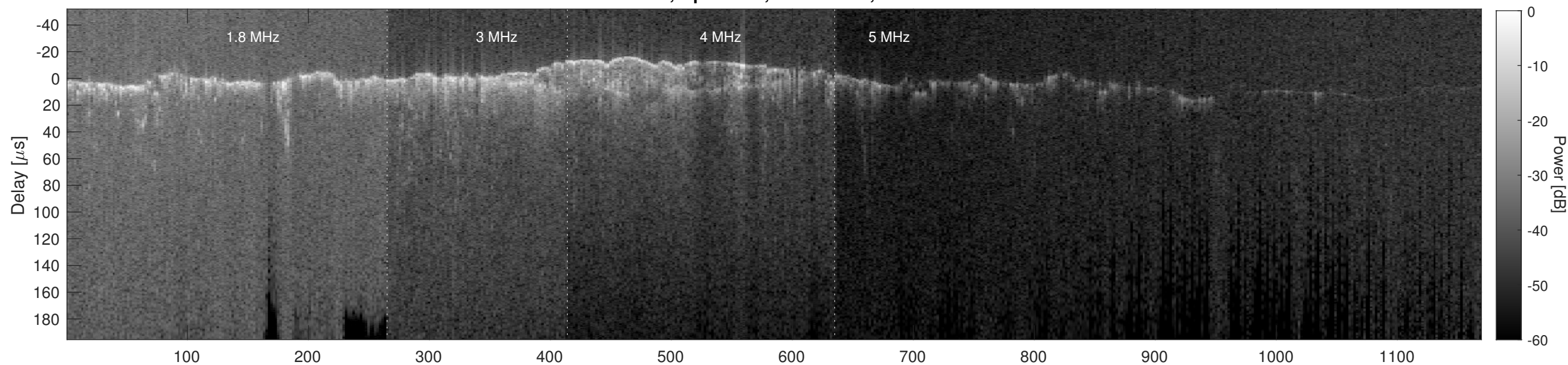
Orbit 2520, Cluttergram
