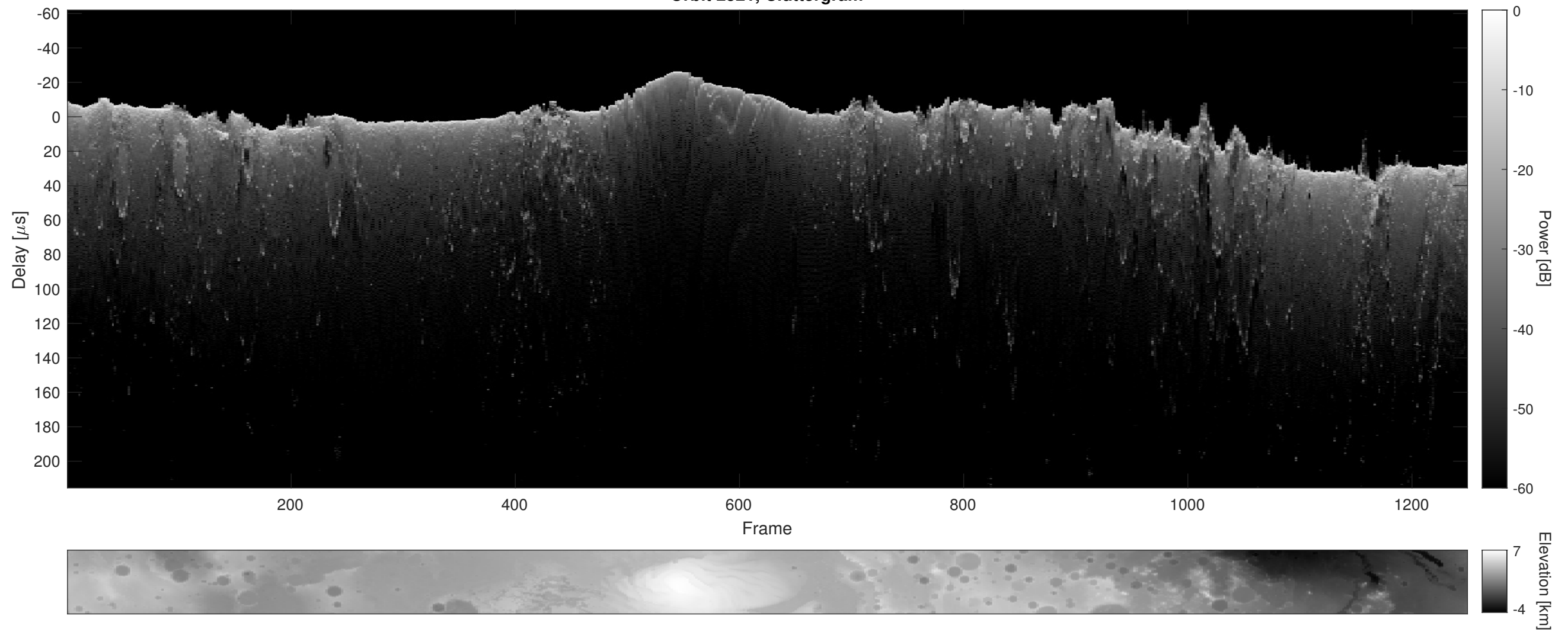
Orbit 2521, Cluttergram
