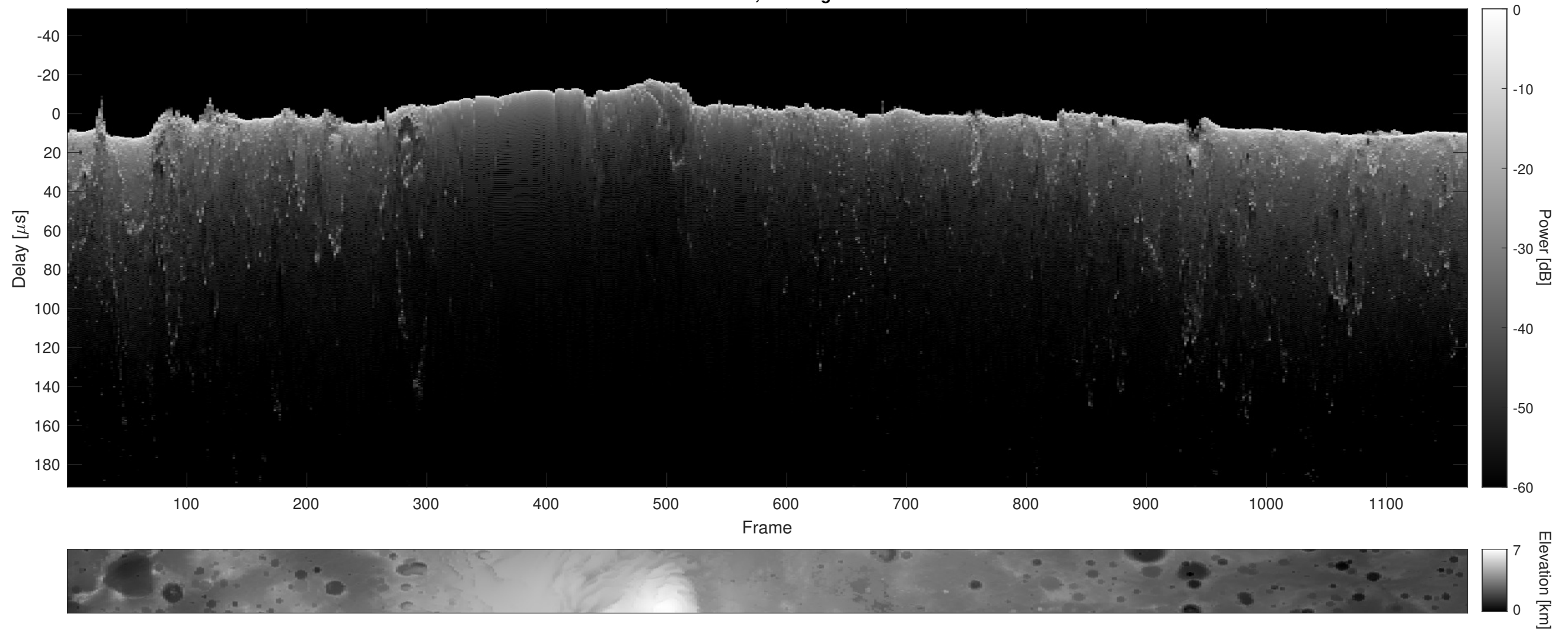
Orbit 2522, Cluttergram
