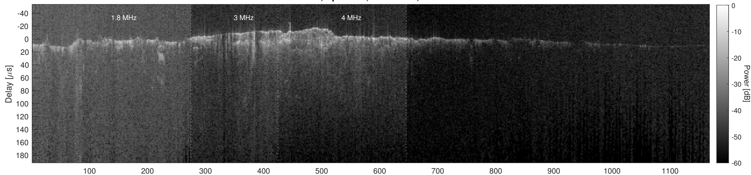
Orbit 2522, Cluttergram
