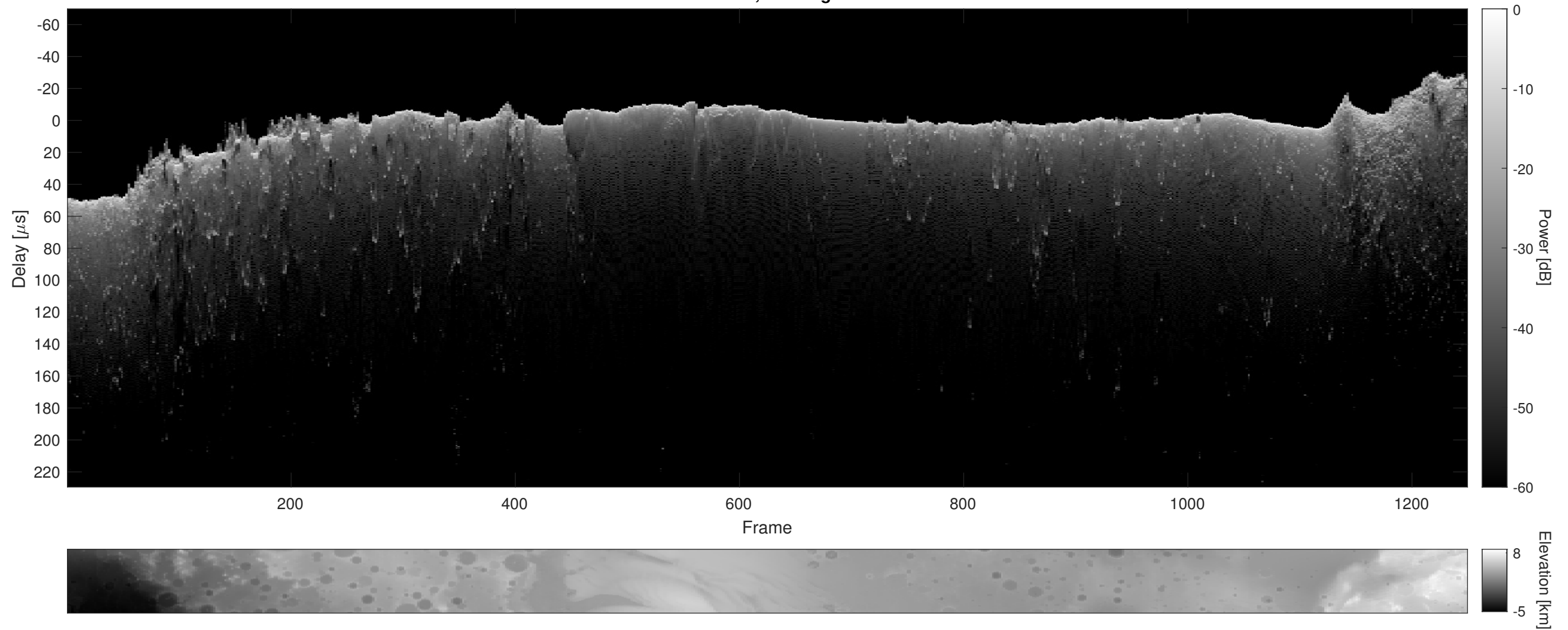
Orbit 2523, Cluttergram
