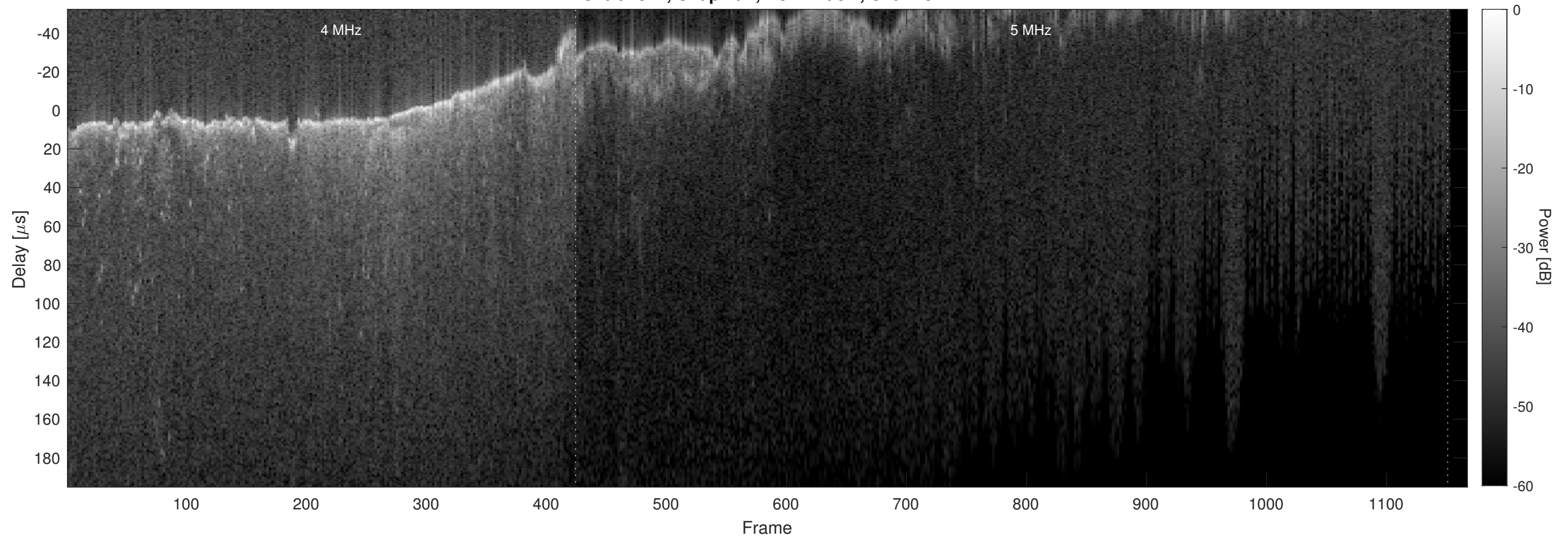
Orbit 2524, Chapman, No Window, Channel 2
