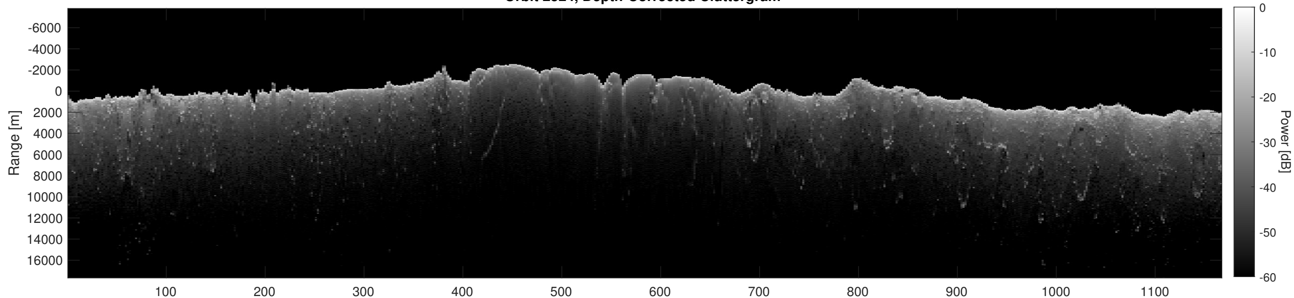
Orbit 2524, Depth-Corrected Cluttergram
