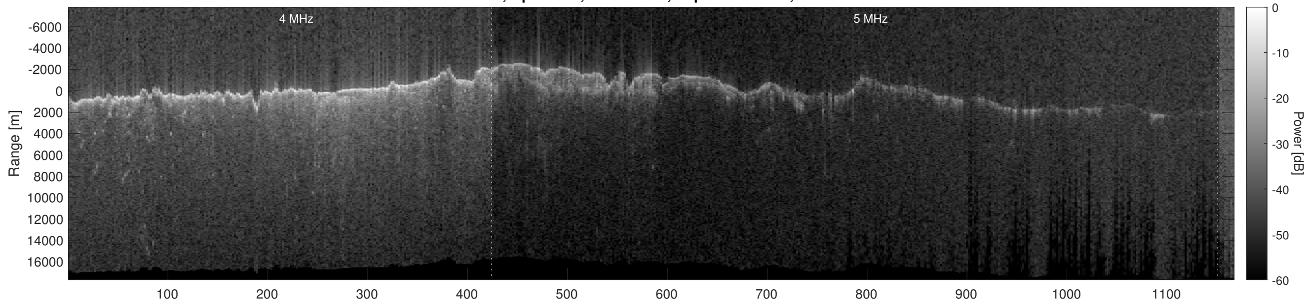
Orbit 2524, Optimized, No Window, Depth-Corrected, Channel 2
