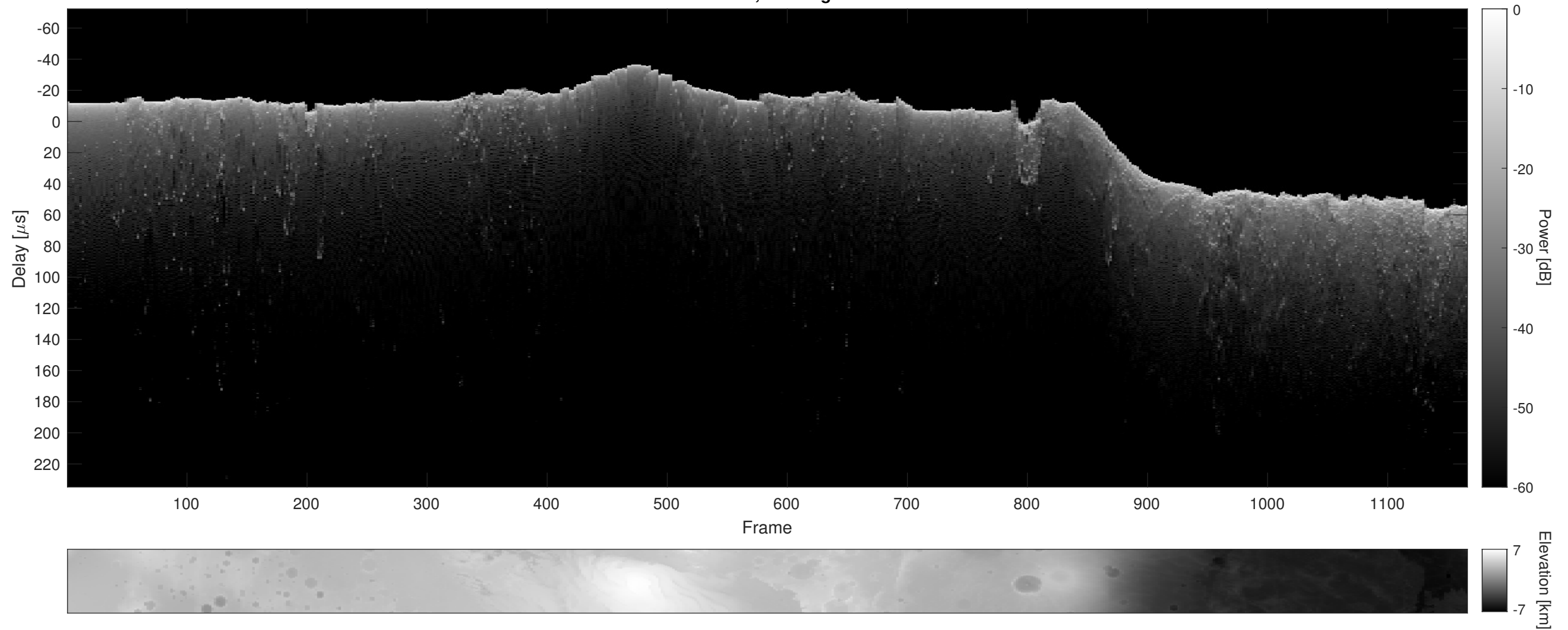
Orbit 2525, Cluttergram
