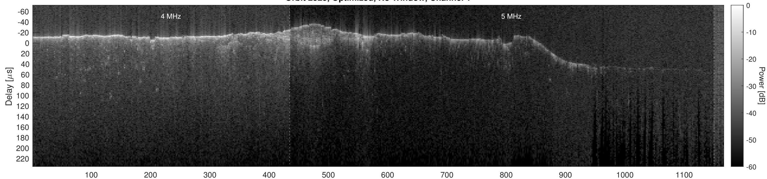
Orbit 2525, Optimized, No Window, Channel 2
