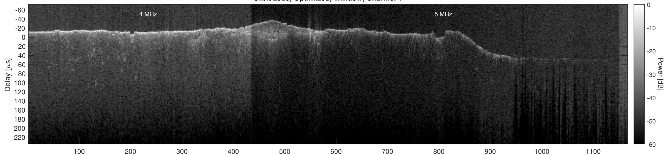
Orbit 2525, Optimized, Window, Channel 2
