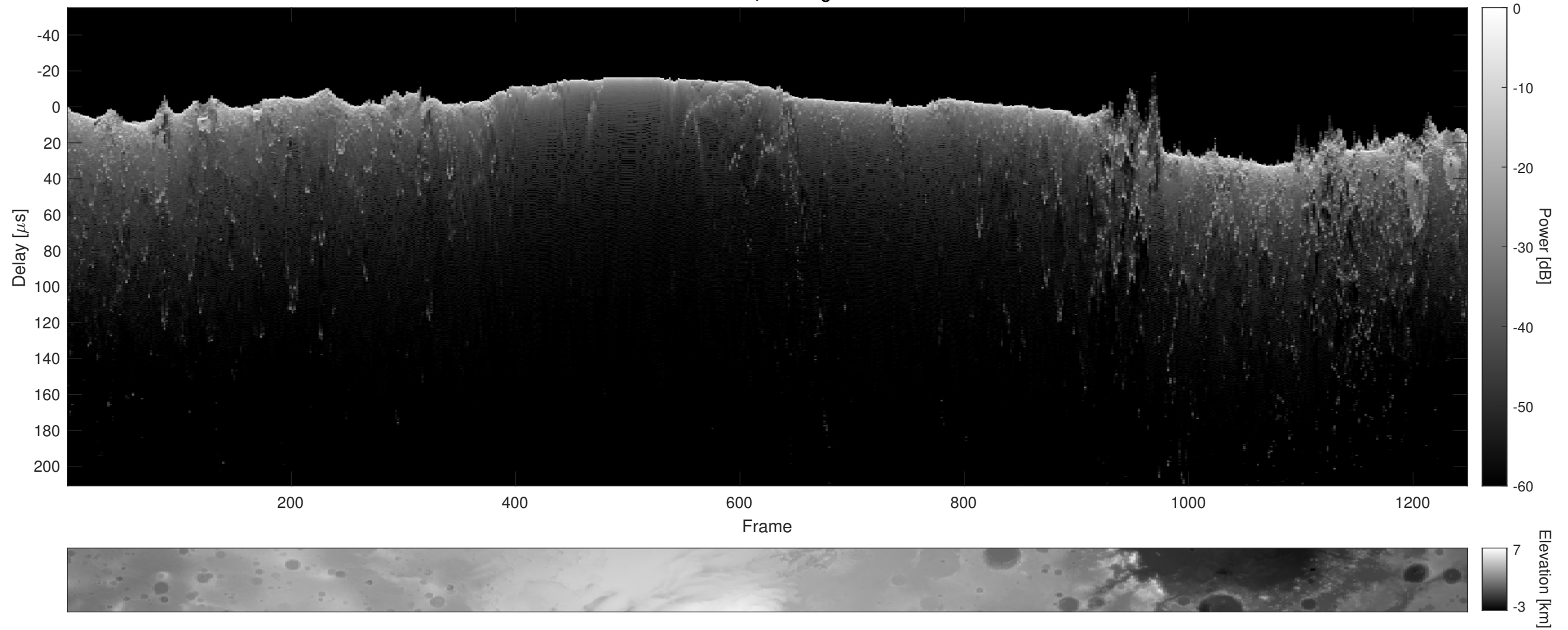
Orbit 2526, Cluttergram
