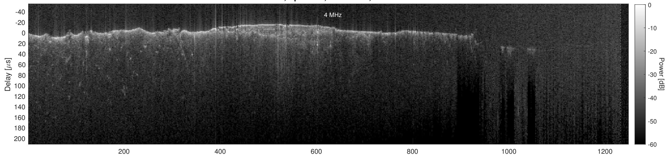
Orbit 2526, Cluttergram
