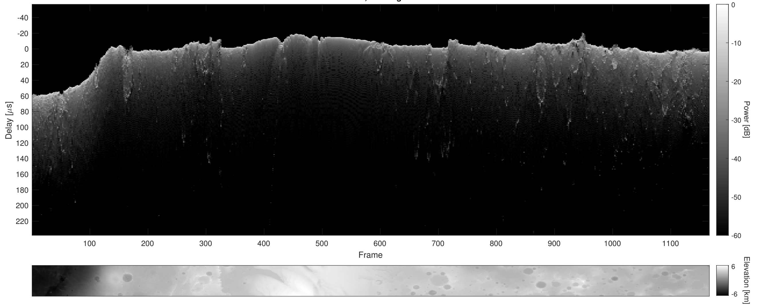
Orbit 2527, Cluttergram
