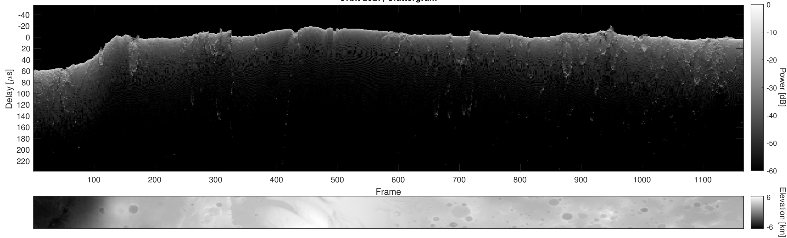
Orbit 2527, Cluttergram
