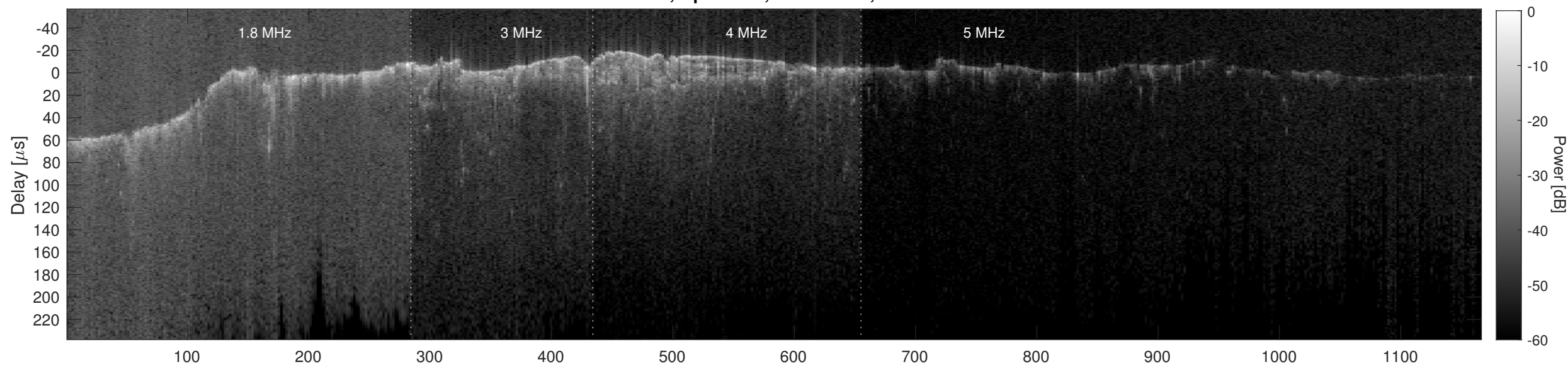
Orbit 2527, Cluttergram
