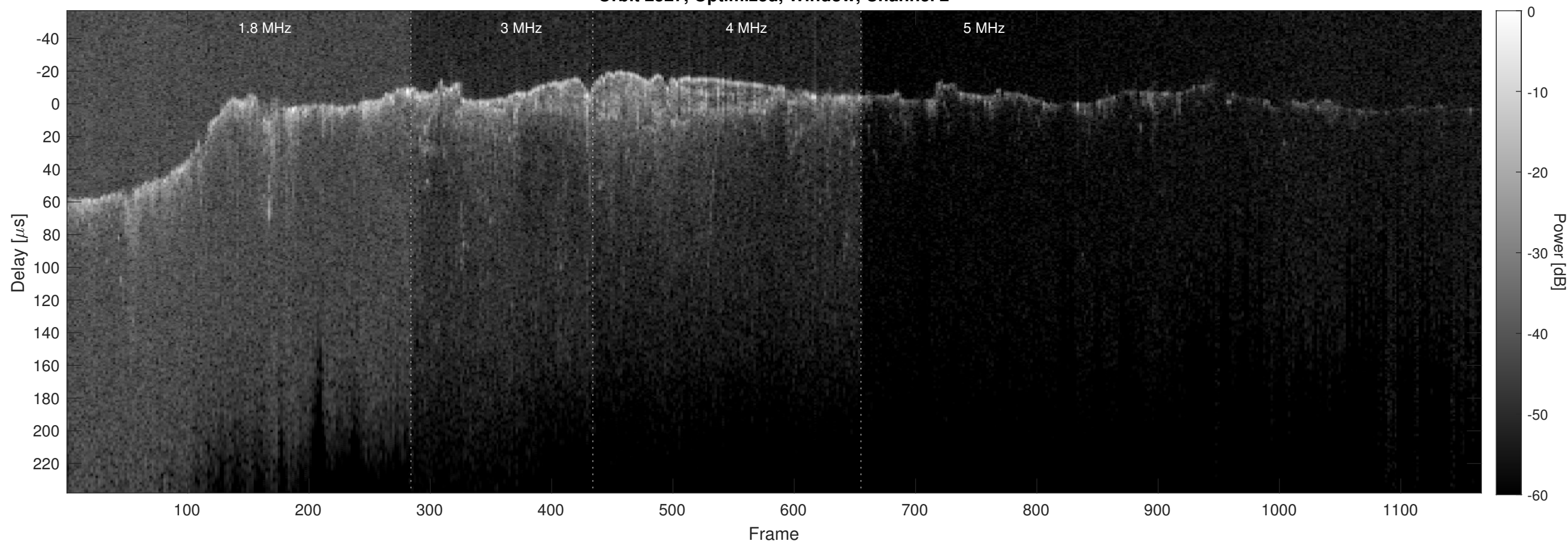
Orbit 2527, Optimized, Window, Channel 2
