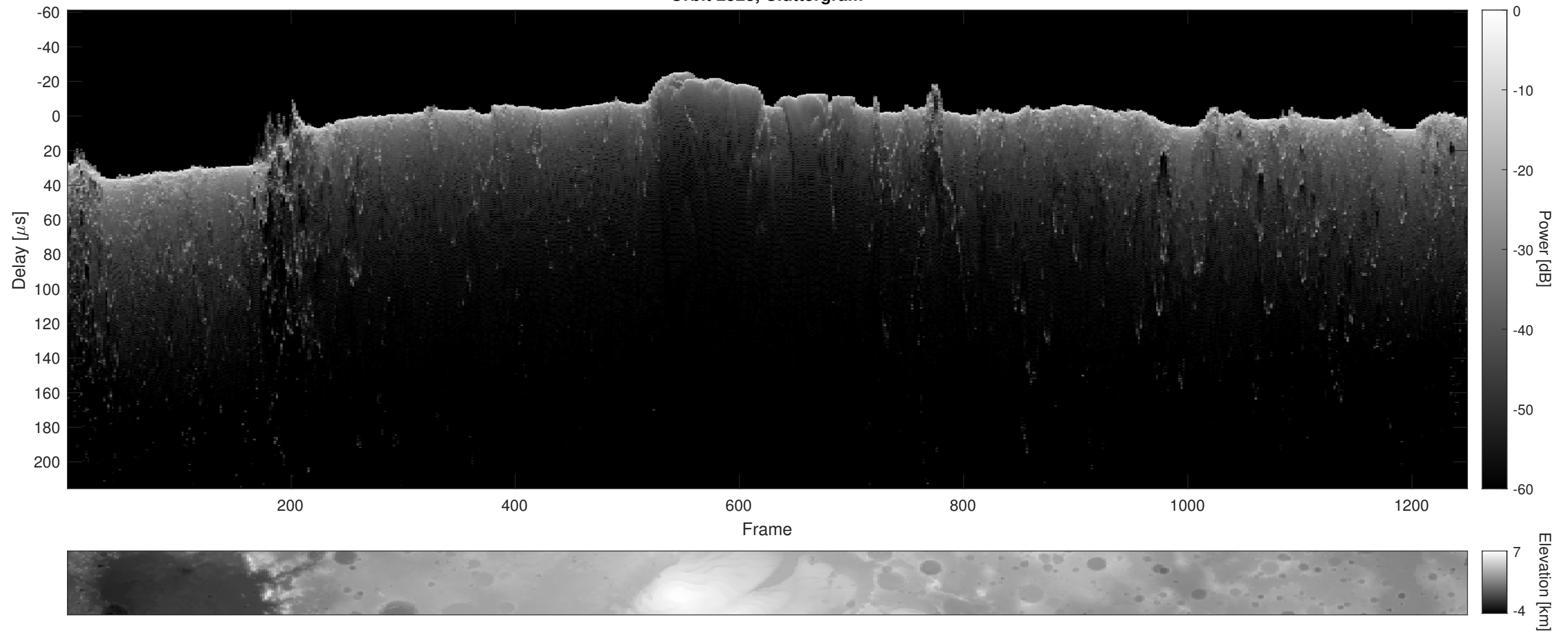
Orbit 2528, Cluttergram
