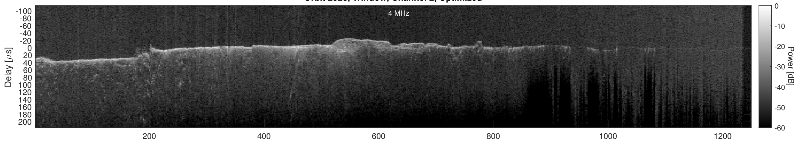
Orbit 2528, Cluttergram
