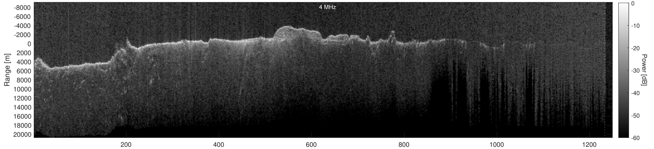
Orbit 2528, Depth-Corrected Cluttergram
