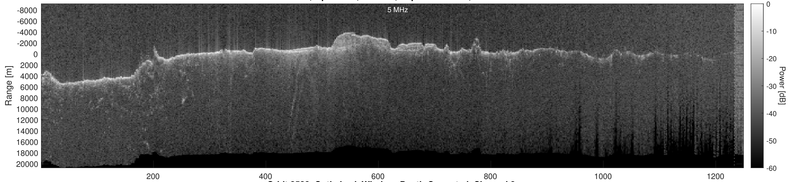
Orbit 2528, Optimized, Window, Depth-Corrected, Channel 2
