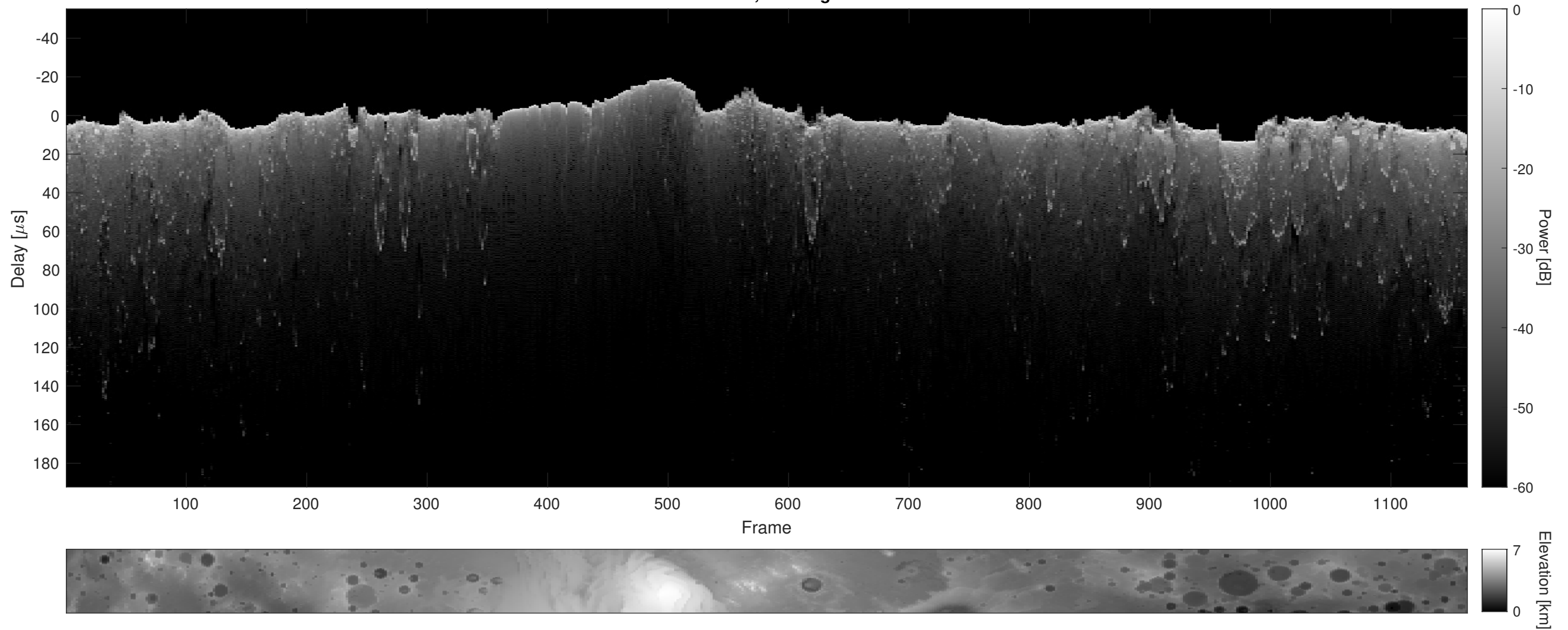
Orbit 2529, Cluttergram
