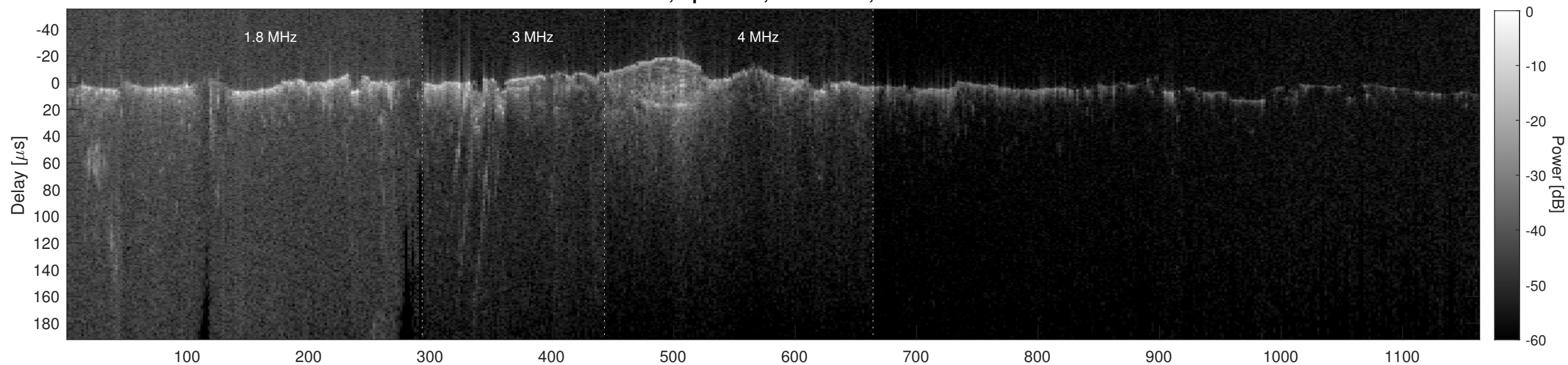
Orbit 2529, Cluttergram
