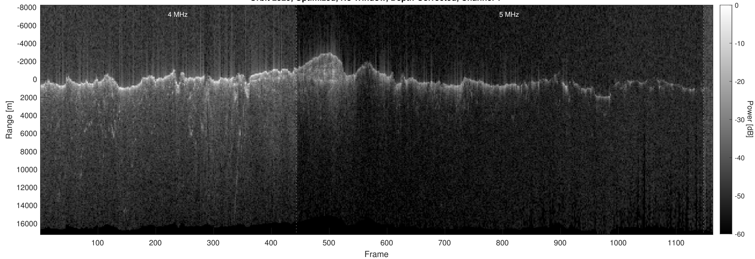
Orbit 2529, Optimized, No Window, Depth-Corrected, Channel 2
