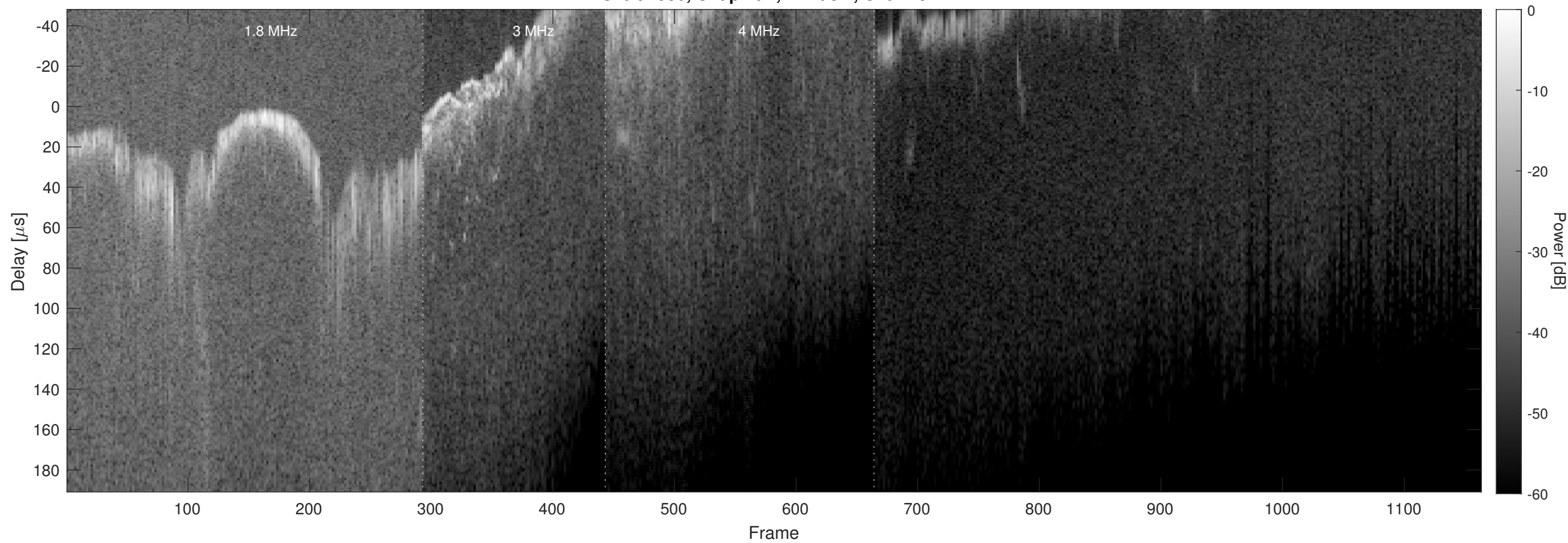
Orbit 2530, Chapman, Window, Channel 2
