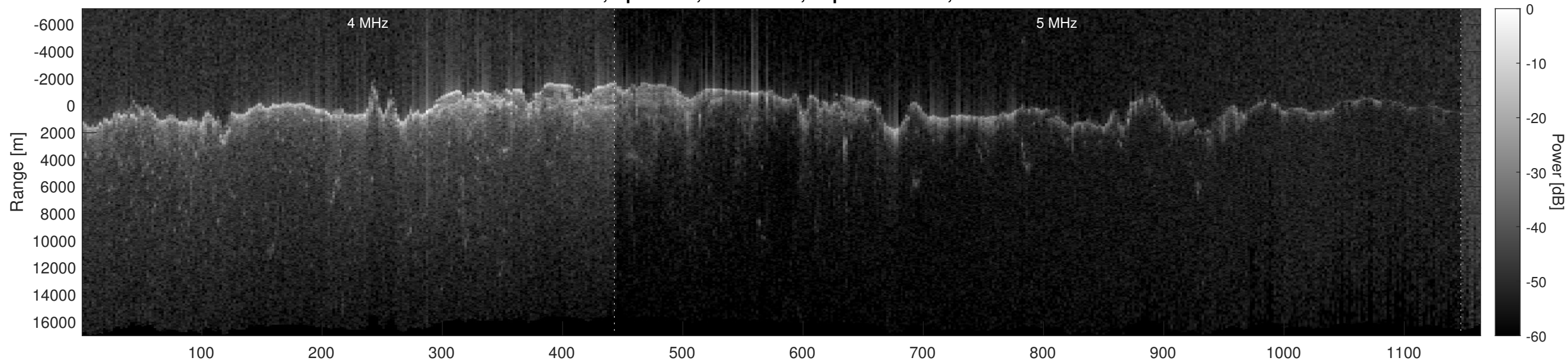
Orbit 2530, Optimized, No Window, Depth-Corrected, Channel 2
