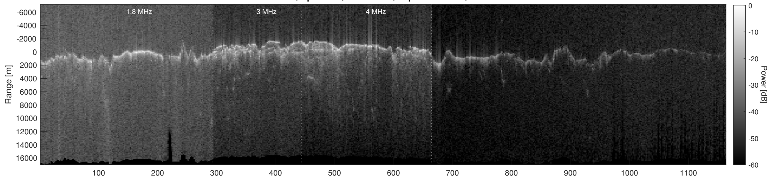
Orbit 2530, Depth-Corrected Cluttergram
