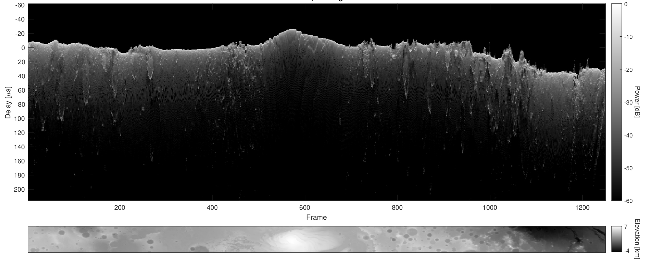
Orbit 2532, Cluttergram
