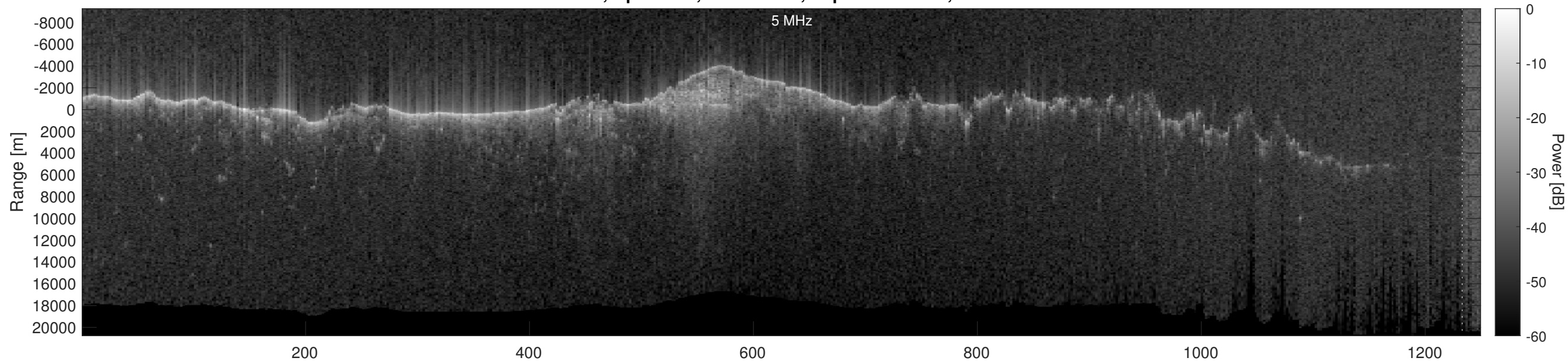
Orbit 2532, Optimized, No Window, Depth-Corrected, Channel 2
