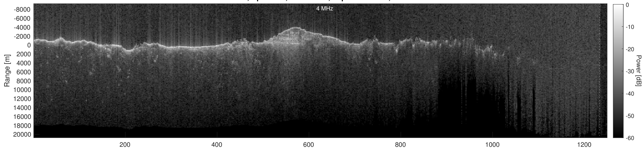
Orbit 2532, Depth-Corrected Cluttergram
