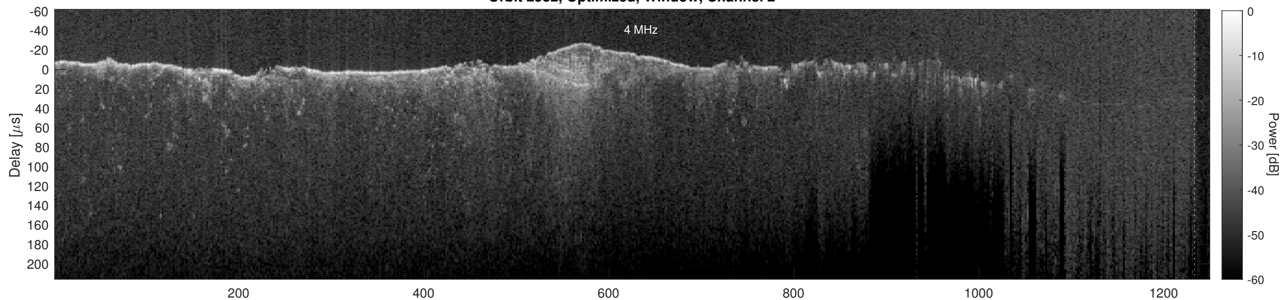
Orbit 2532, Cluttergram
