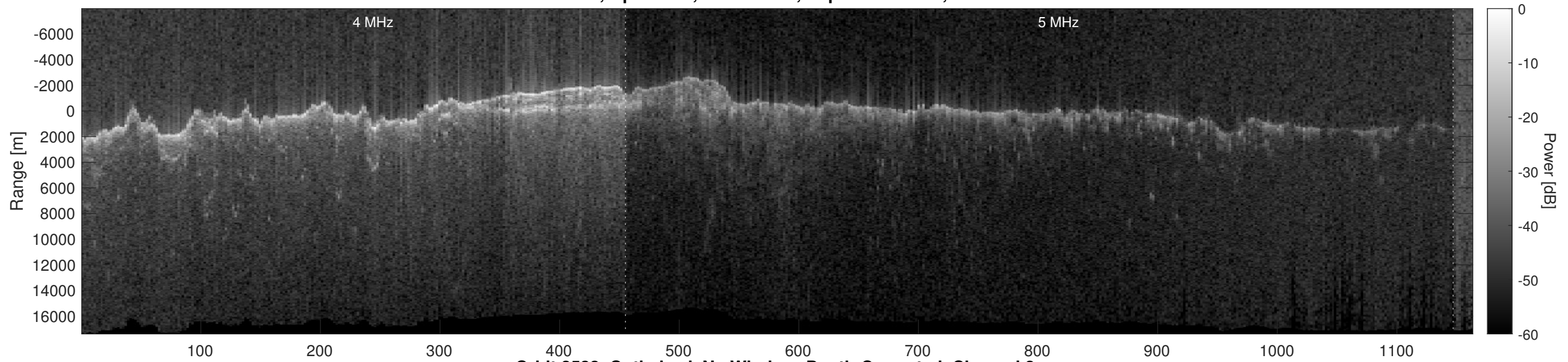
Orbit 2533, Optimized, No Window, Depth-Corrected, Channel 2
