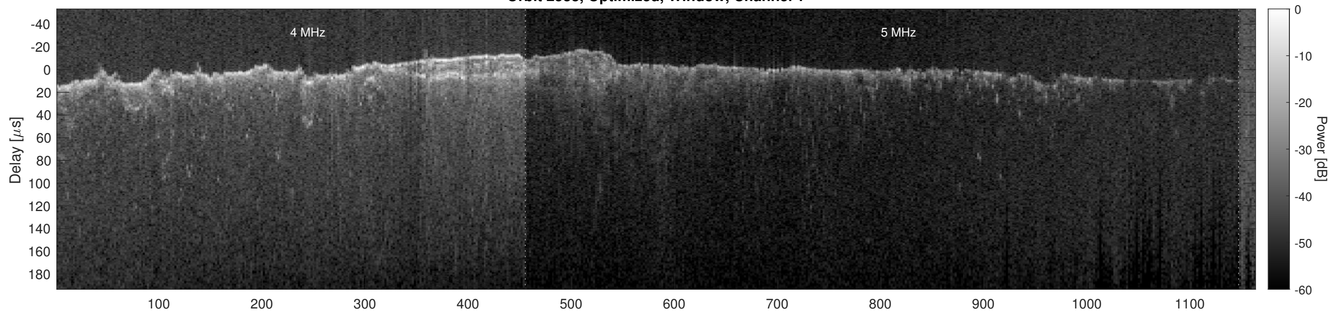
Orbit 2533, Optimized, Window, Channel 2
