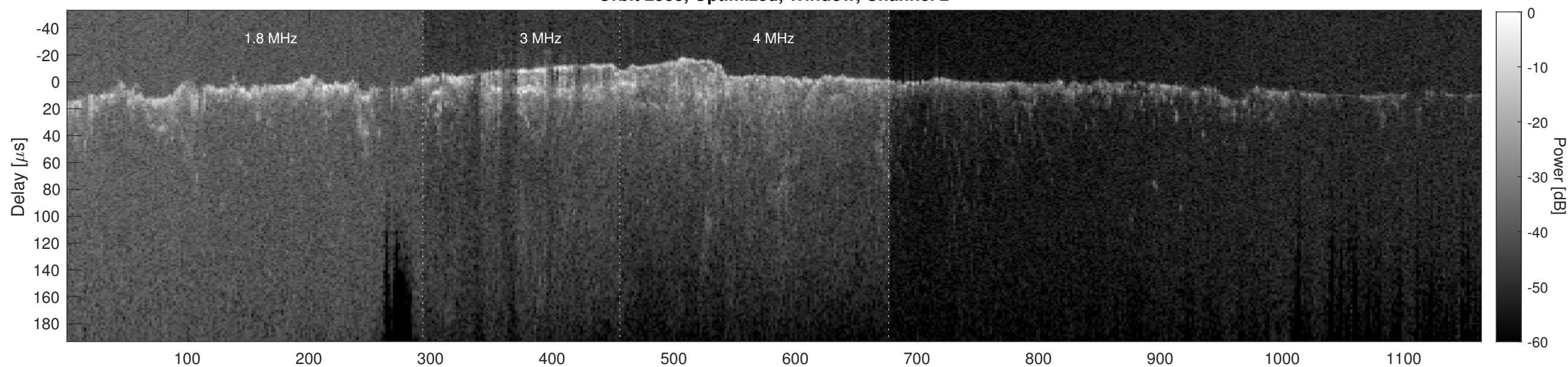
Orbit 2533, Cluttergram
