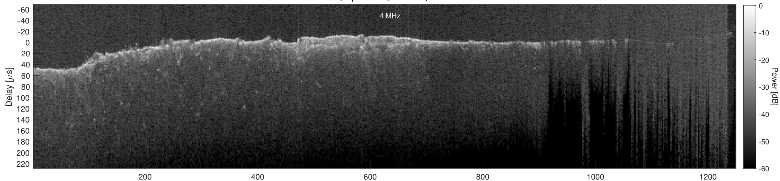
Orbit 2534, Cluttergram
