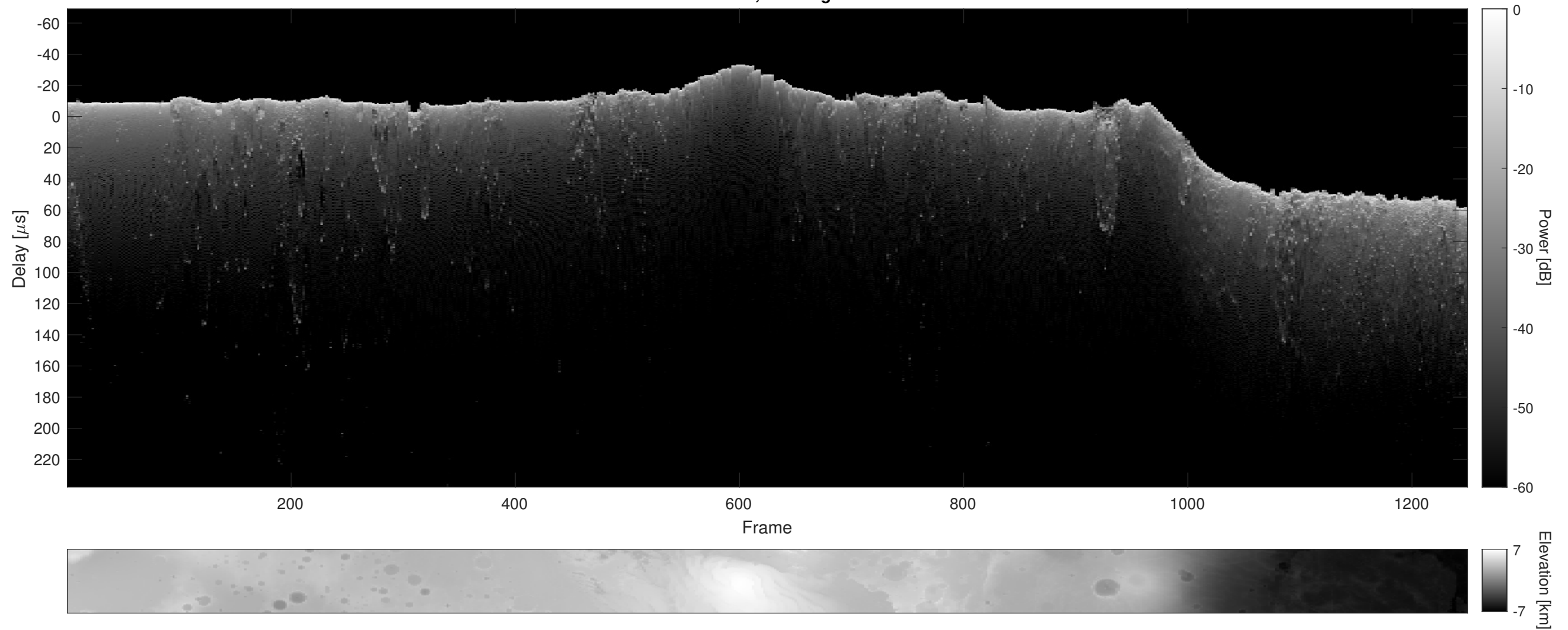
Orbit 2536, Cluttergram
