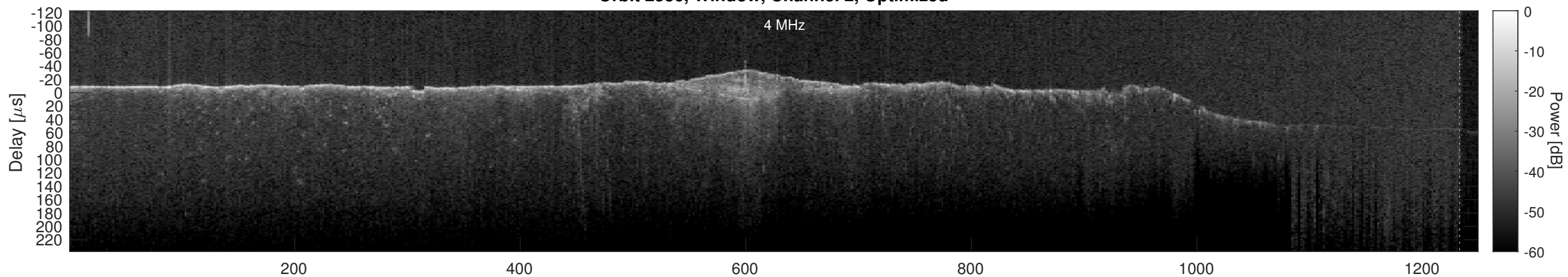
Orbit 2536, Cluttergram
