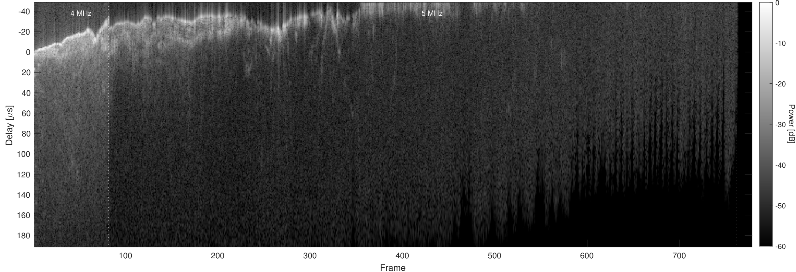
Orbit 2538, Chapman, No Window, Channel 2
