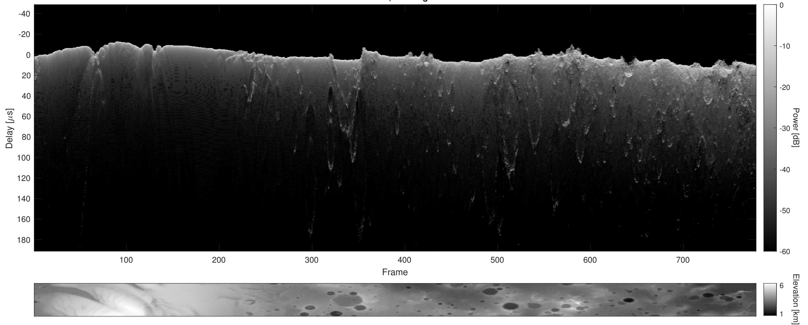
Orbit 2538, Cluttergram
