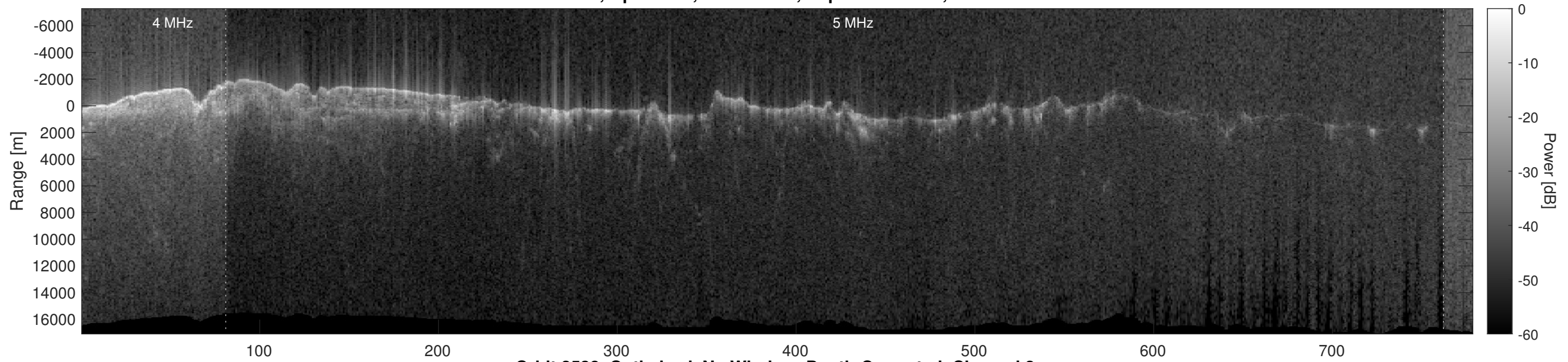
Orbit 2538, Optimized, No Window, Depth-Corrected, Channel 2
