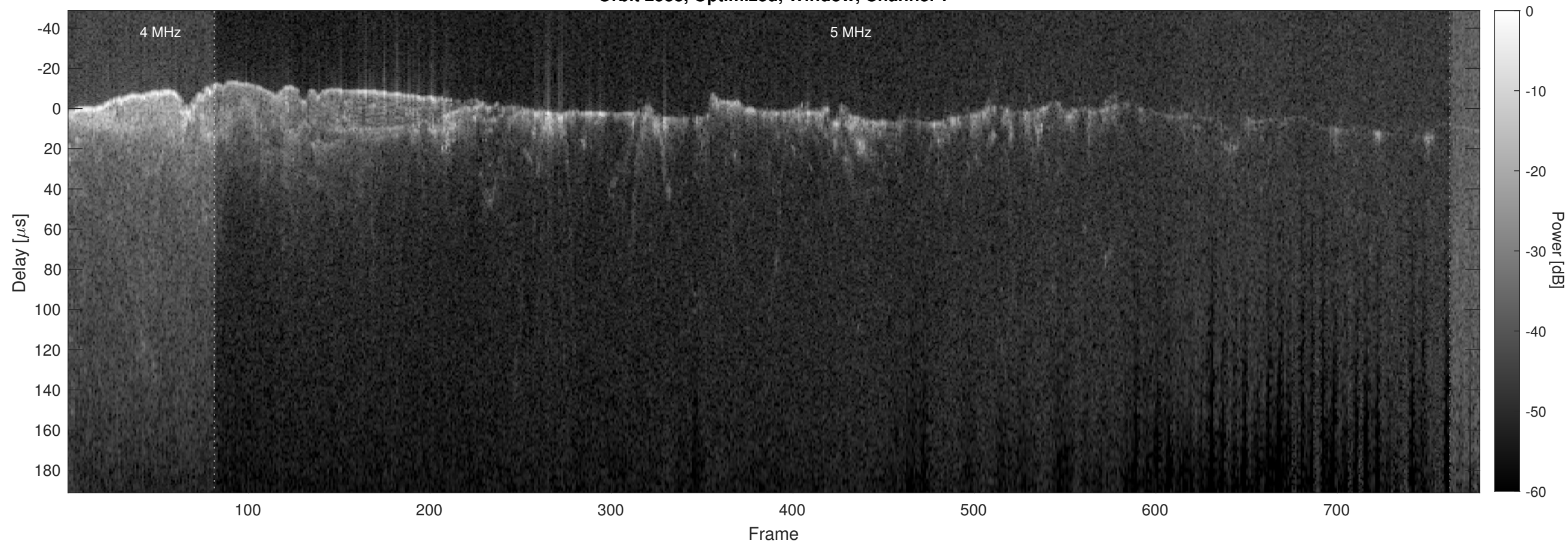
Orbit 2538, Optimized, Window, Channel 2
