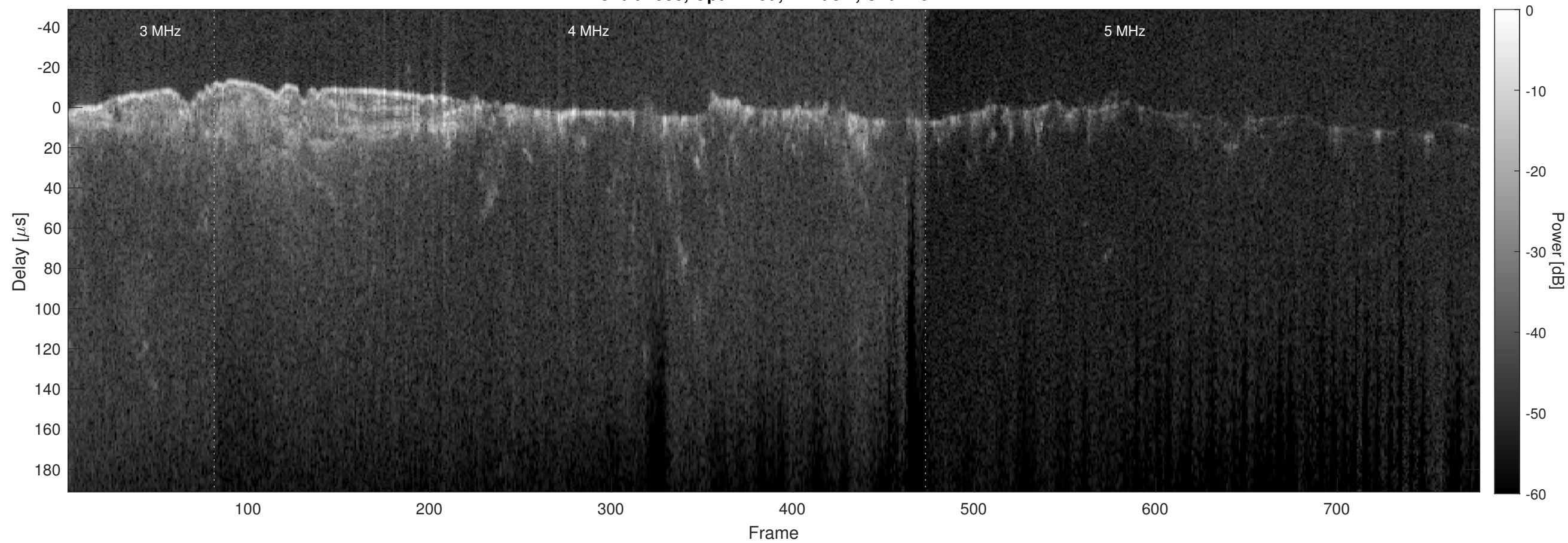
Orbit 2538, Optimized, Window, Channel 2
