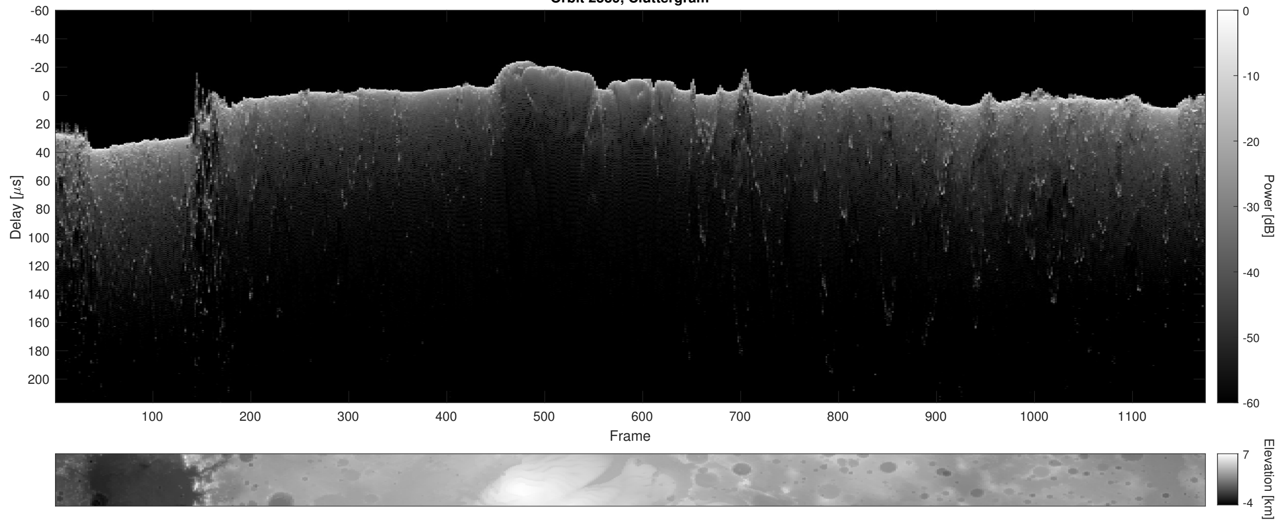
Orbit 2539, Cluttergram
