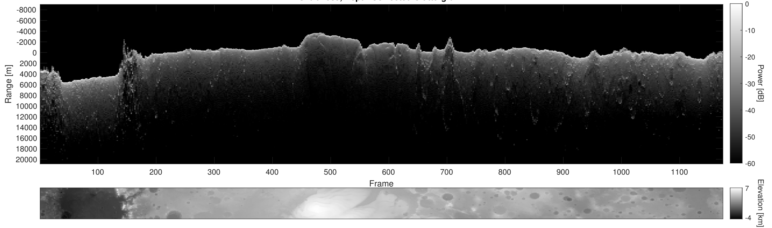
Orbit 2539, Depth-Corrected Cluttergram
