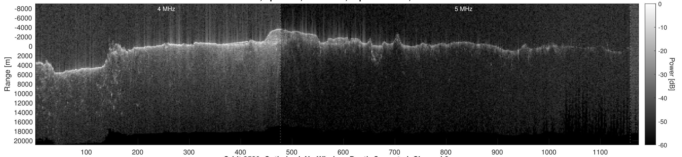
Orbit 2539, Optimized, No Window, Depth-Corrected, Channel 2
