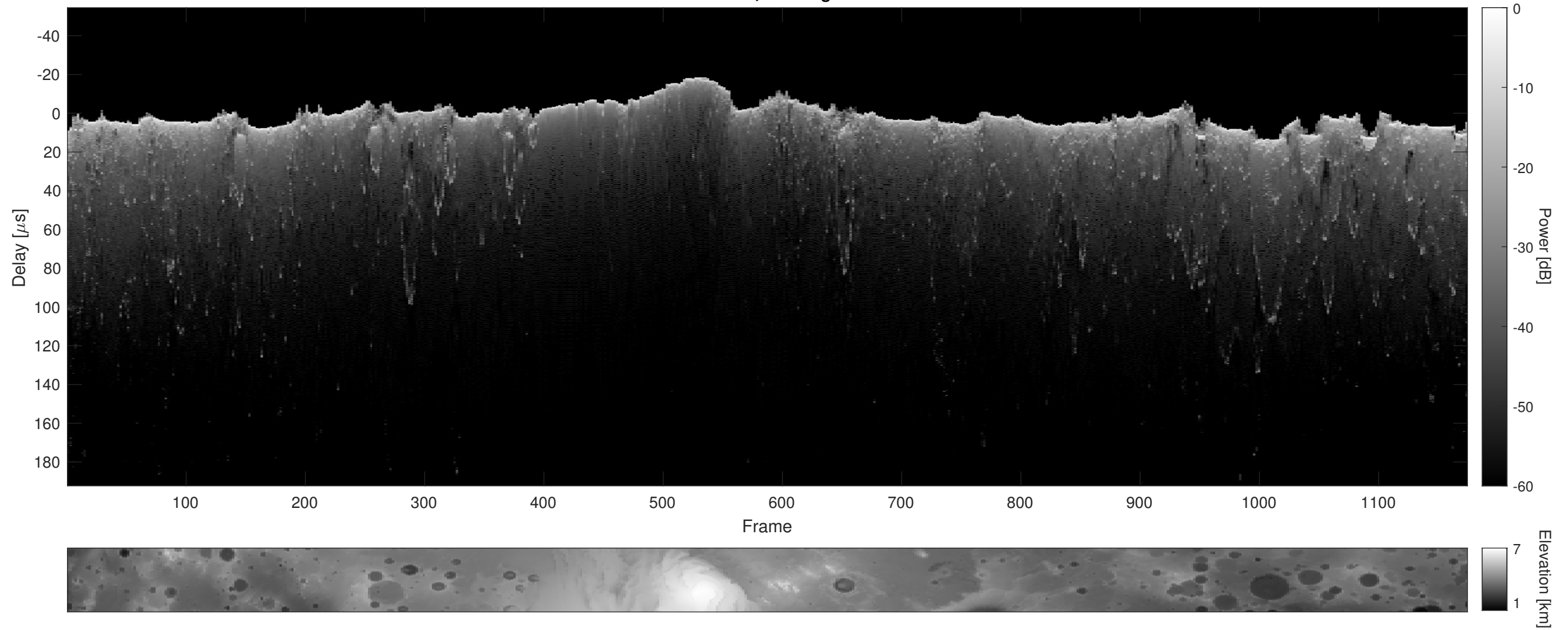
Orbit 2540, Cluttergram
