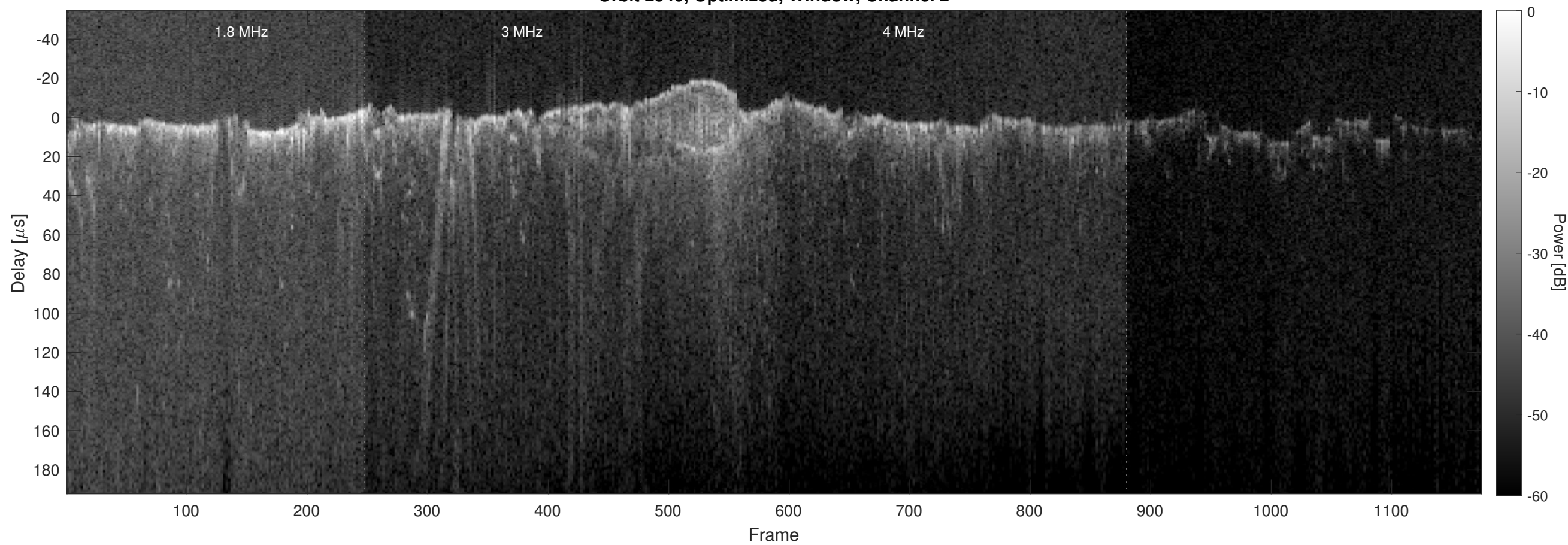
Orbit 2540, Optimized, Window, Channel 2
