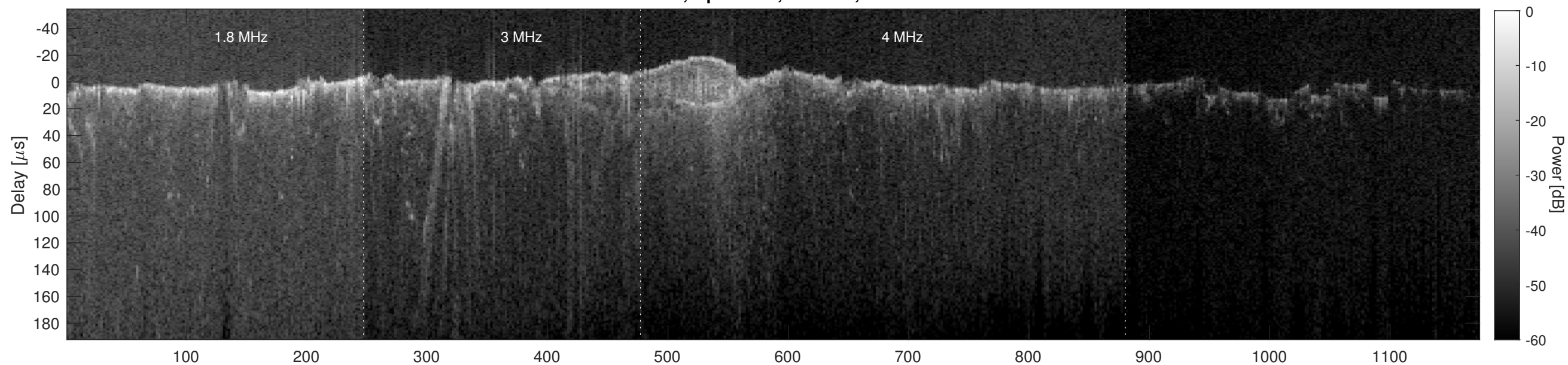
Orbit 2540, Cluttergram
