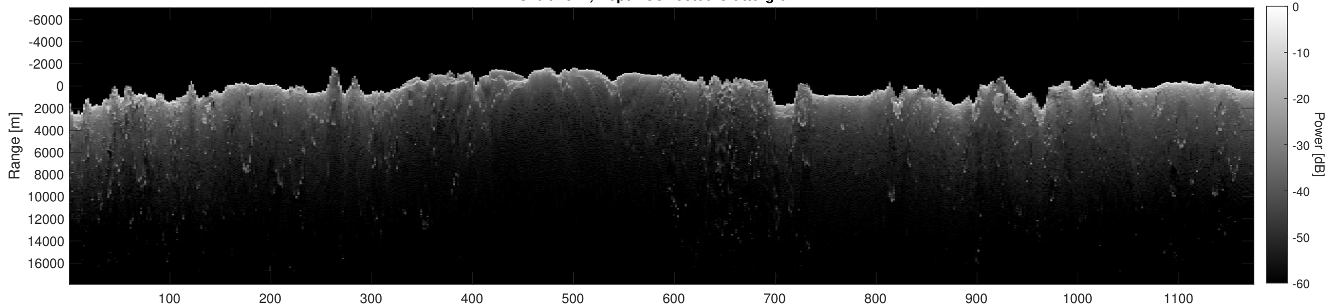
Orbit 2541, Depth-Corrected Cluttergram
