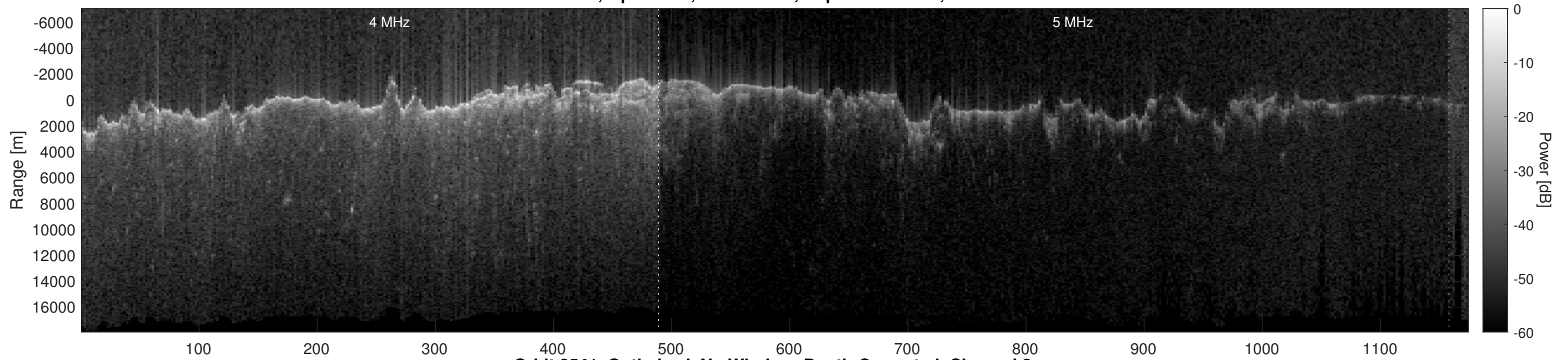
Orbit 2541, Optimized, No Window, Depth-Corrected, Channel 2
